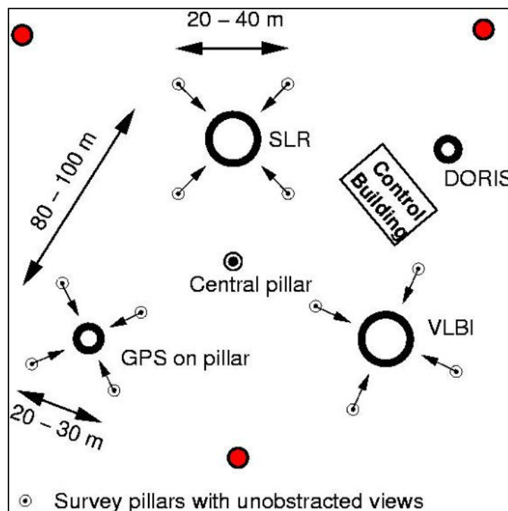
Figure 4. Conceptual Layout of the Local Area Geodetic Markers; dimensions included just to give a rough estimate of scale
