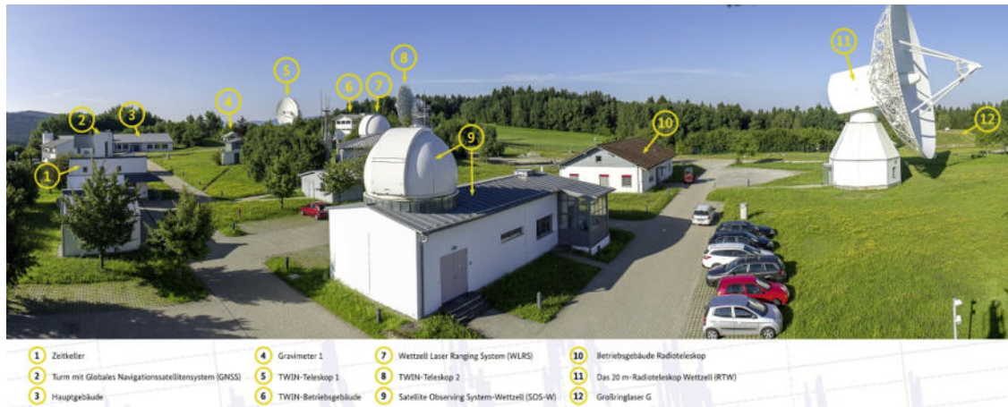
Figure 2b. Core Site at Wettzell, Germany
